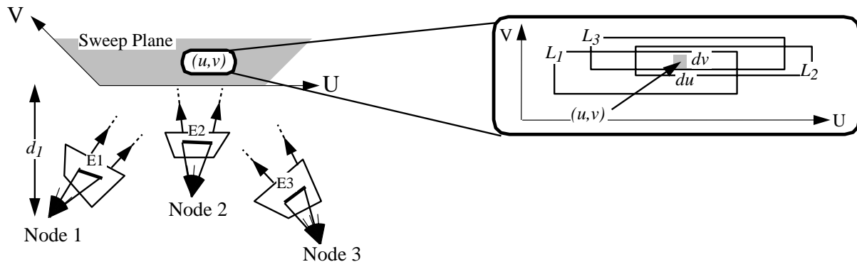
Figure 4: Parameters in the correlation function. The figure on the left shows edges E_1 , E_2 , and E_3 from three nodes projected onto a plane. The figure on the right is a blowup of a small section of the plane. It depicts overlap of the rectangles L_1 , L_2 , and L_3 corresponding to the edges.
